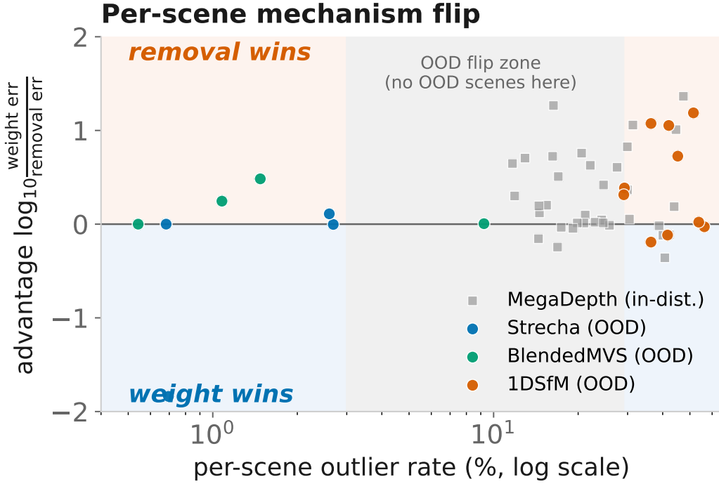
Figure 5: Per-scene complementarity (RESfM-aligned schedule). Each point is one scene: outlier rate (x, log) vs. signed advantage of removal over soft weighting. Weight wins at low contamination, removal at high contamination.
