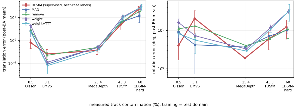
Figure 3: The completed in-distribution contamination curve. Post-BA mean translation (log scale) when training and test share the domain, versus measured track contamination. The supervised recipe uses best-case labels (GT-derived; on MegaDepth, its native COLMAP labels). Each label-free arm is its own line: soft weighting ( \pm TTT) leads at low contamination, robust removal (madweight, remove) at high — the complementarity mechanism flip replicated in-distribution. Supervision wins at 0.5% and 25% and narrowly at 43%, and loses at 3.1% (dataset-specific dead zone) and 60% (the causal label ceiling): its failures are two distinct modes, not a smooth function of contamination. The rotation panel (right) tells the same story and makes the BlendedMVS dead zone starker still (supervised 20.7 \pm 12.2^\circ vs. label-free 4\text{--}13^\circ ). Bands: \pm std over five training seeds (Olsson: two; MegaDepth rotation: five-seed means, bands omitted).
